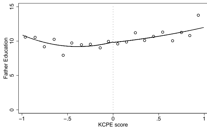
Figure 4: RD Validity: local quadratic regressions of covariates on KCPE scores.
