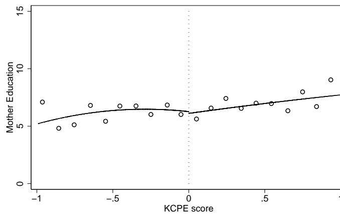
Figure 4: RD Validity: local quadratic regressions of covariates on KCPE scores.
